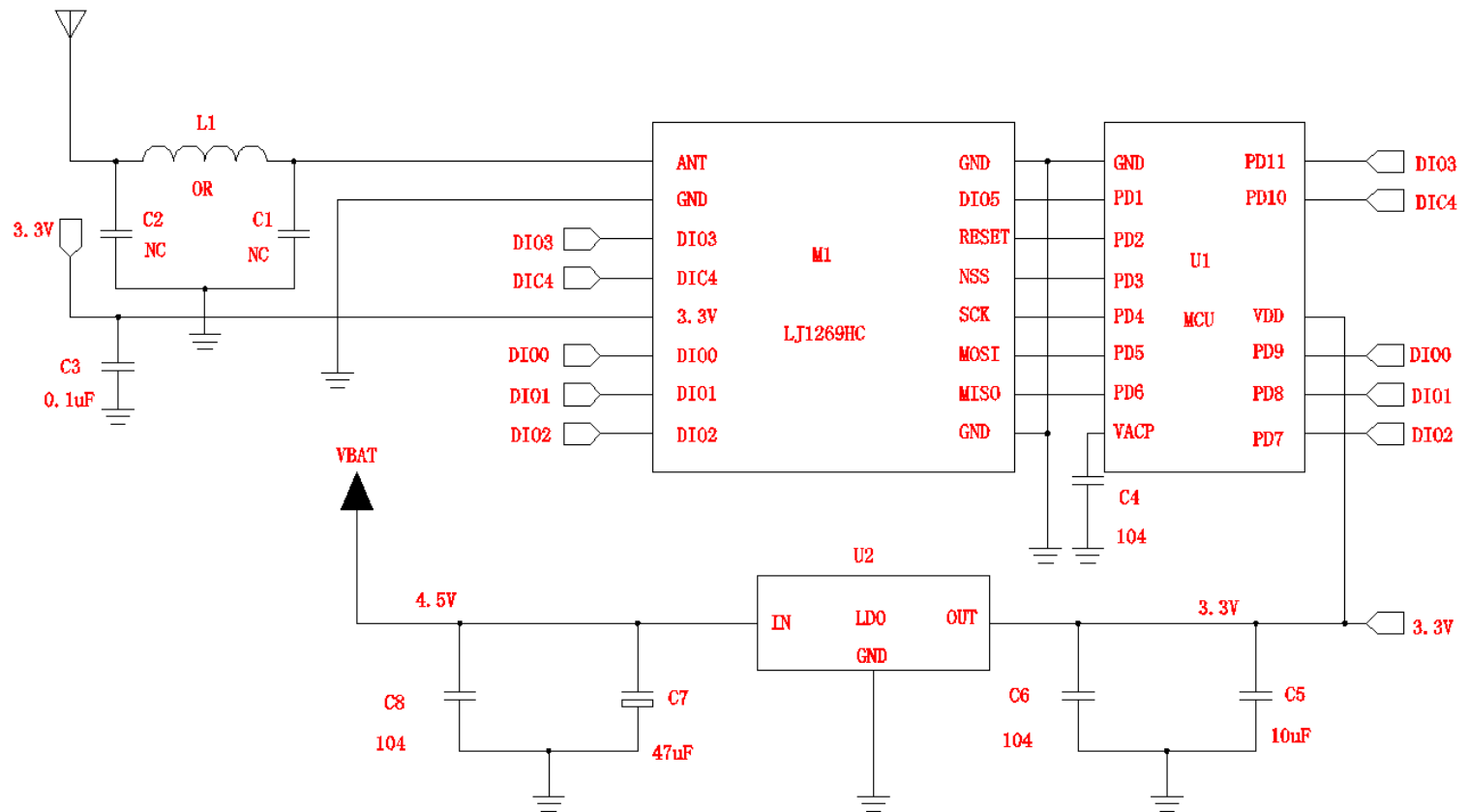
Figure 40. Typical Application Schematic
