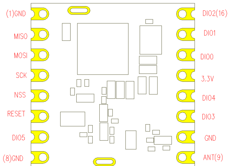
Figure 2. Marking Diagram
