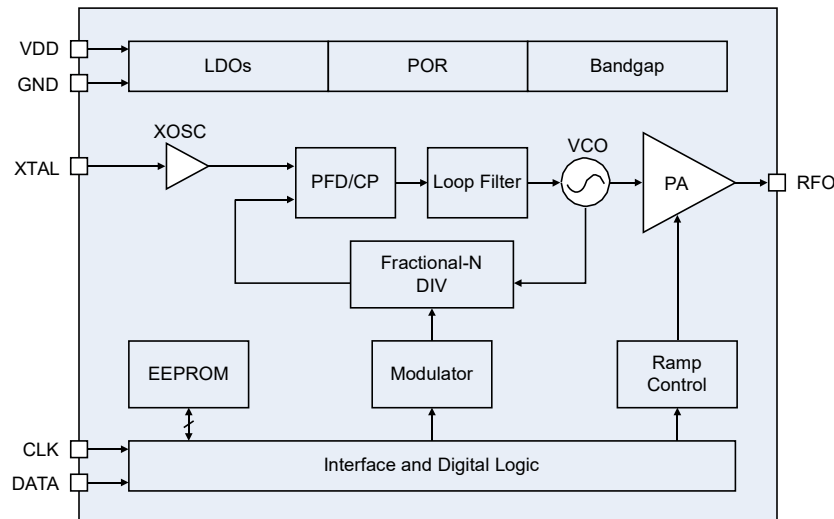
Figure 8. MD220 Functional Block Diagram
