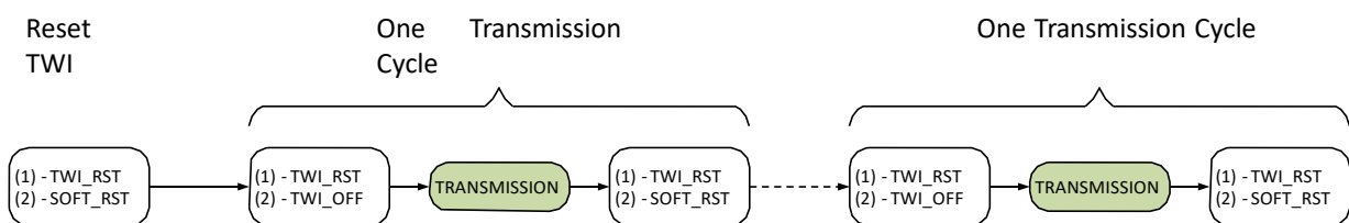
Figure 16. MD220 Operation Flow with TWI
