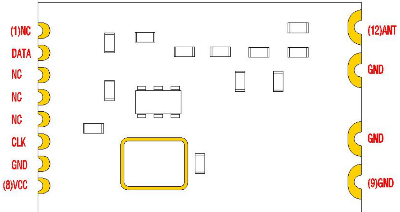
Figure 1. Pin Configuration
